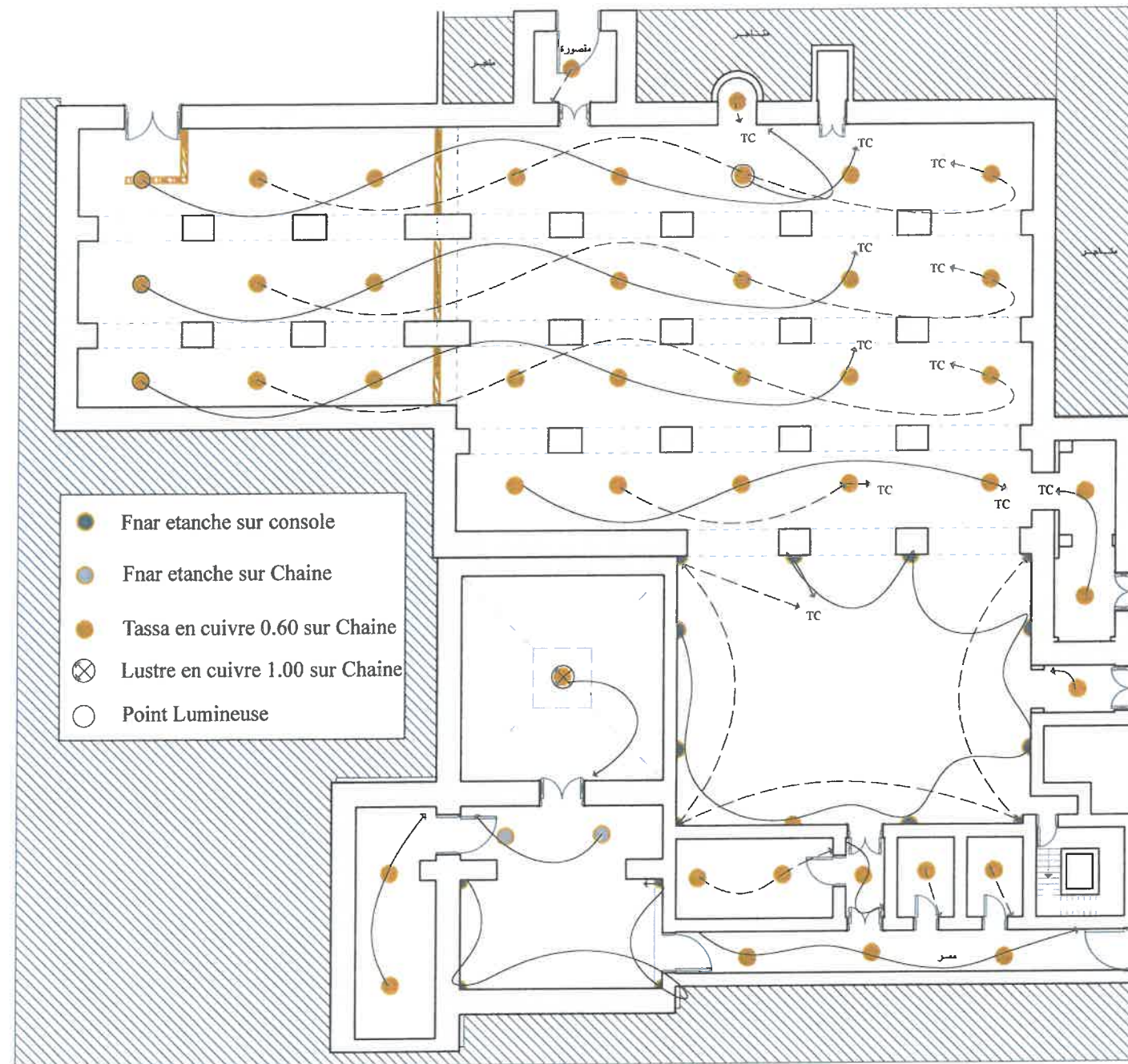
RDC REPERAGE ELECTRIQUE
