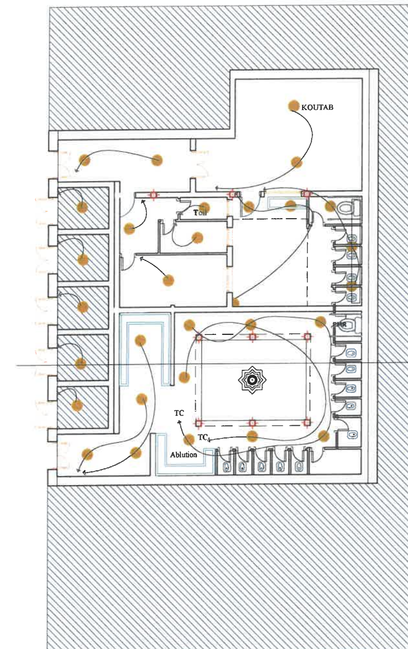
ABLUTIONS REPERAGE ELECTIQUE
