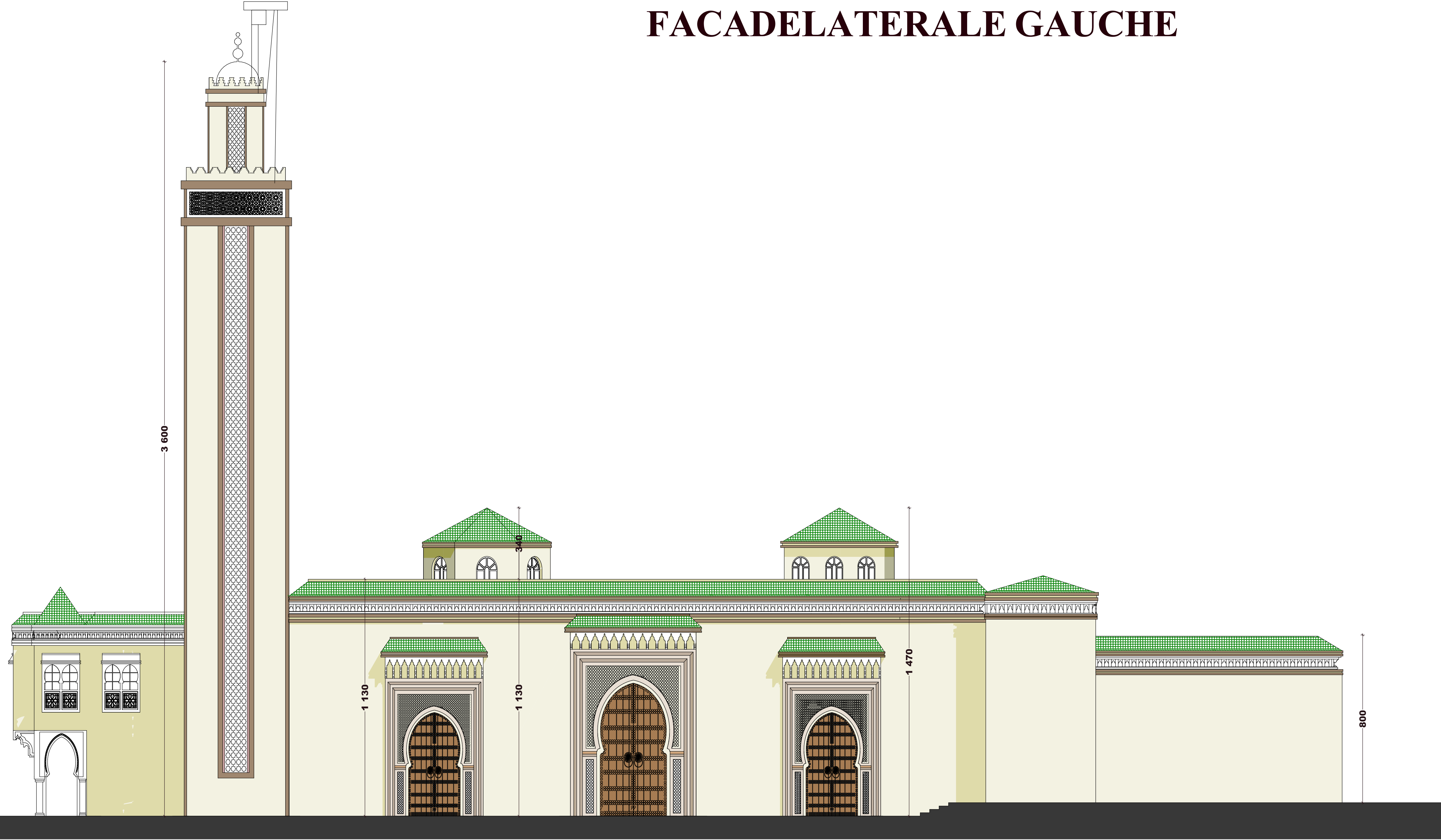
FACADE ARRIERE
